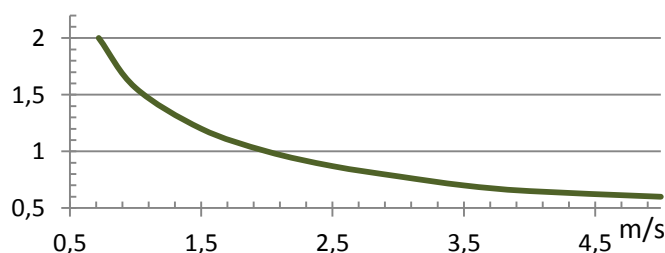
Graph 3: R_{th,f} / R_{th,f} (2 \text{ m/s})
