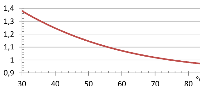
Graph 2: R_{th,n} / R_{th,n} (\Delta T = 75^{\circ}C)
